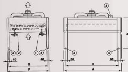
Horizontal installation
